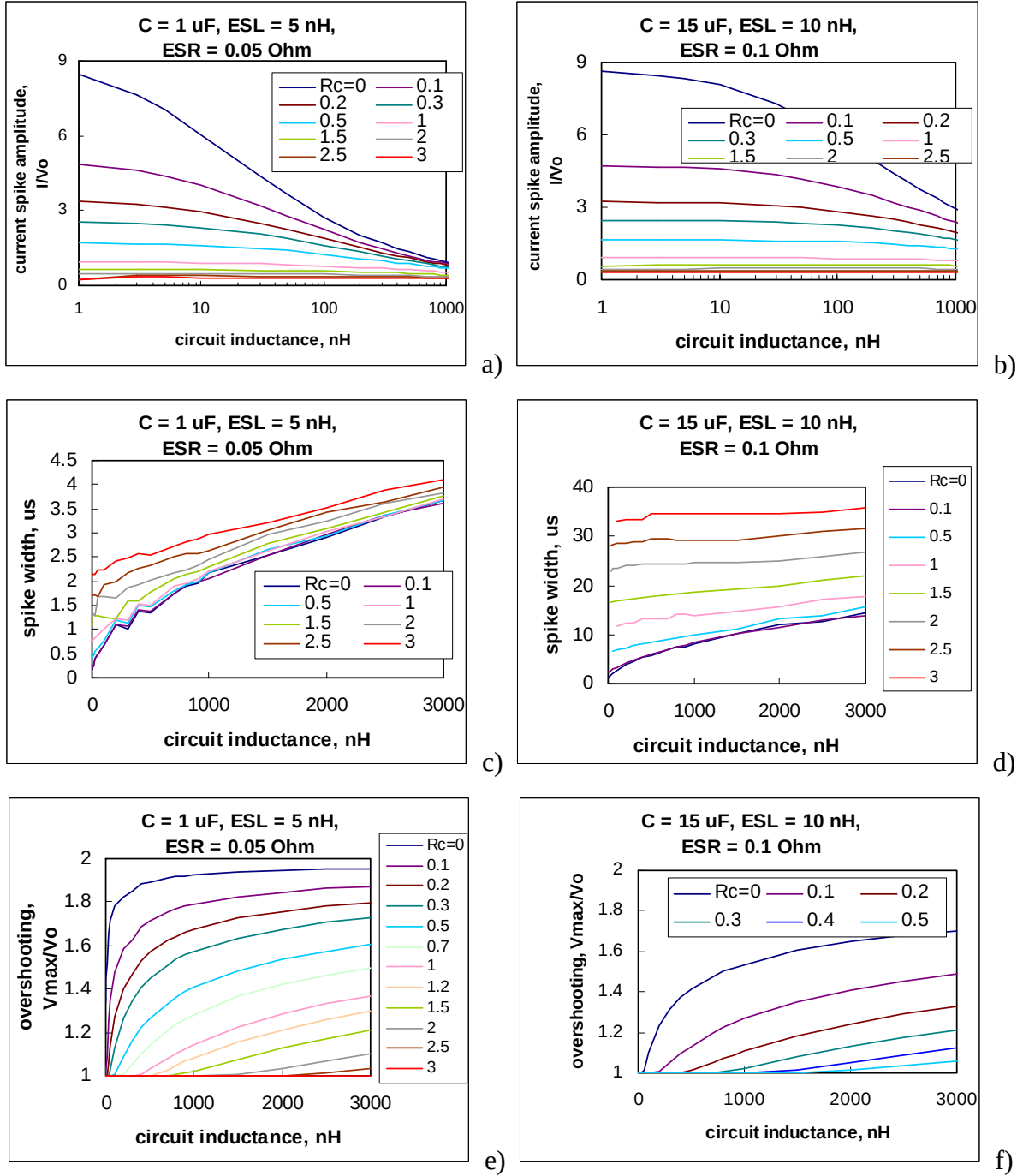
Figure 8. Effect of inductance and resistance of the circuit on the amplitude of current spike (a, b), spike duration (c, d), and overshooting (e, f) for a 1 \mu\text{F} (a, c, e) and 15 \mu\text{F} (b, d, f) capacitors. The legend shows values of R_c in Ohms.
